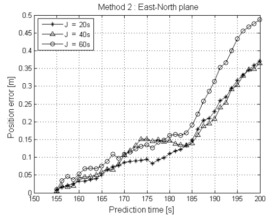
Figure 17: Error for GPS outage at t = 155[s] . a) Method 1, b) Method 2.
