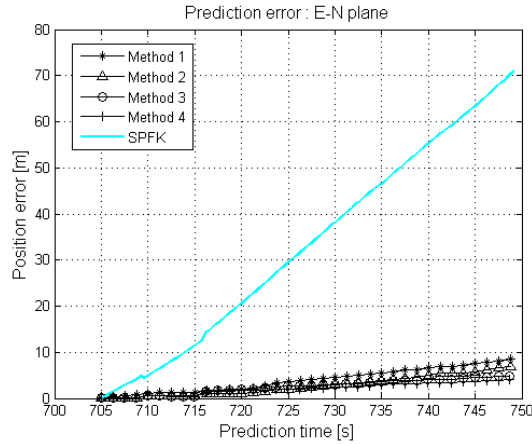
Figure 21: Error for GPS outage at t = 705[s] .
